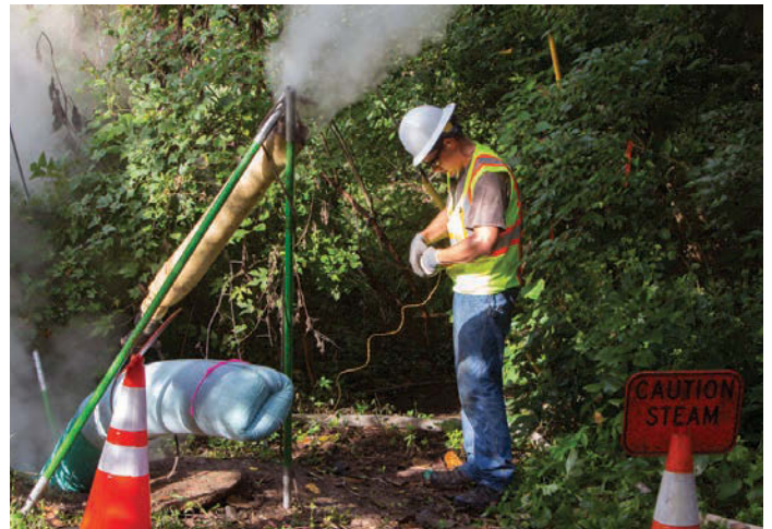
Kyle Bowen, an SAK crew foreman, connects a temperature monitoring wire to an inverted CIPP liner at the start of the curing process.
